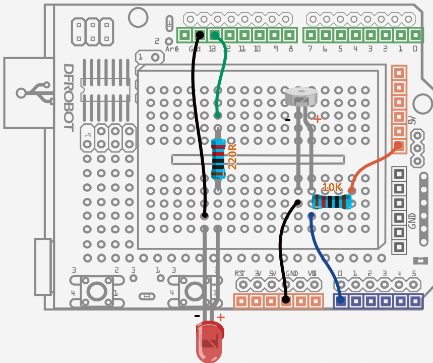
Diagram of the photo diode circuit
