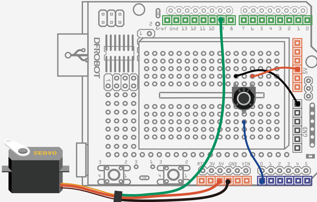
Fig. 11-1 Controllable Servo Circuit Diagram
