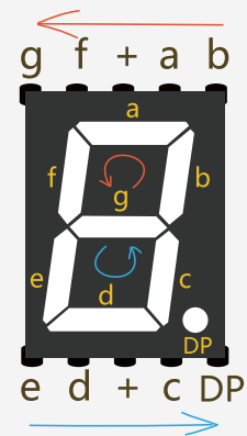
Fig. 15-2 Pin-out Instructions
