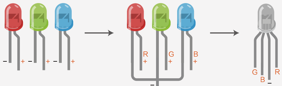
Fig. 5-2 How 3 LEDs form A RGB LED (Common Cathode)
