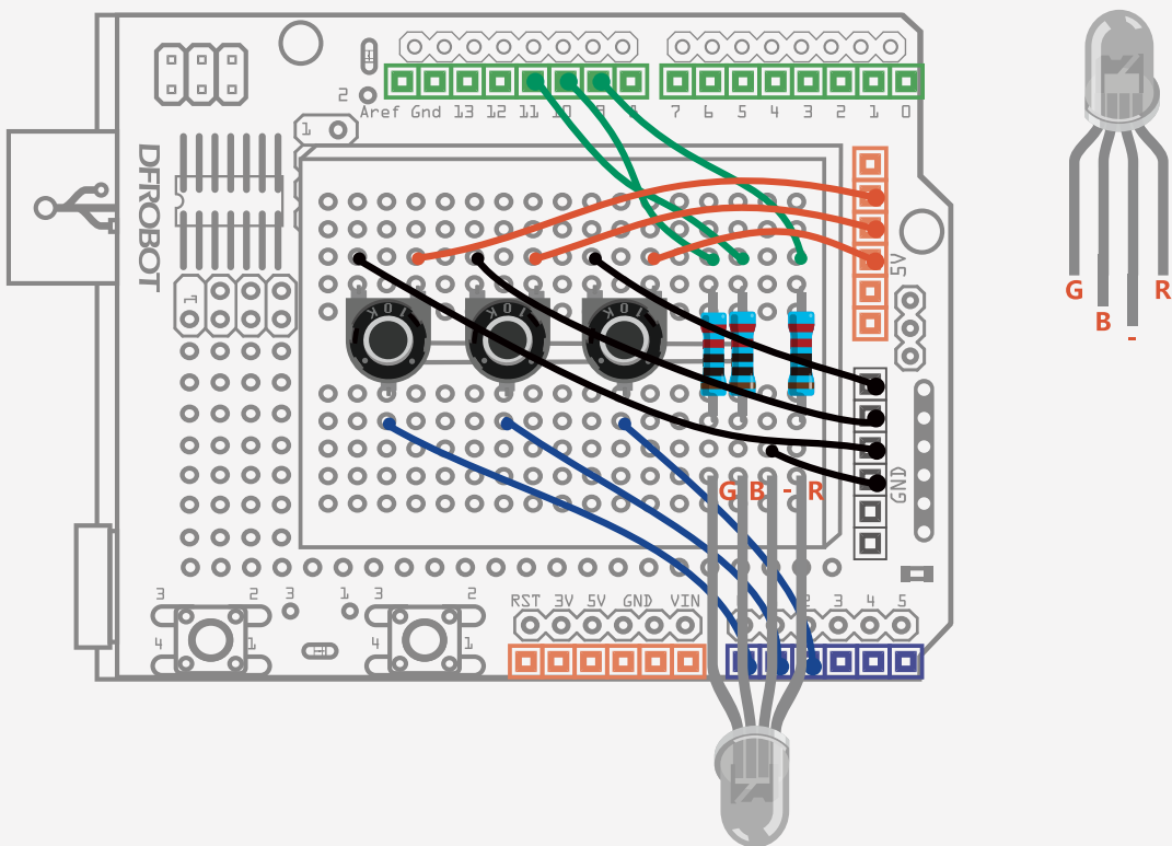
Fig. 12-1 Interactive Adjustable RGB LED Circuit diagram
