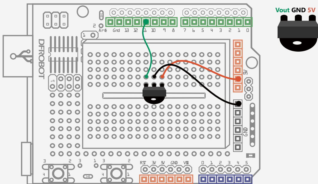
Fig. 14-1 IR Receiver Diagram
