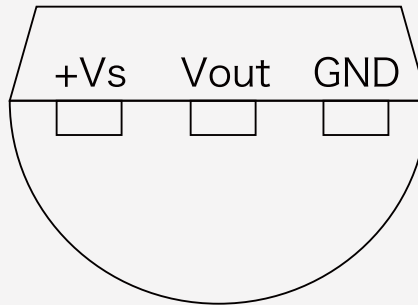
Diagram of LM35 pins
