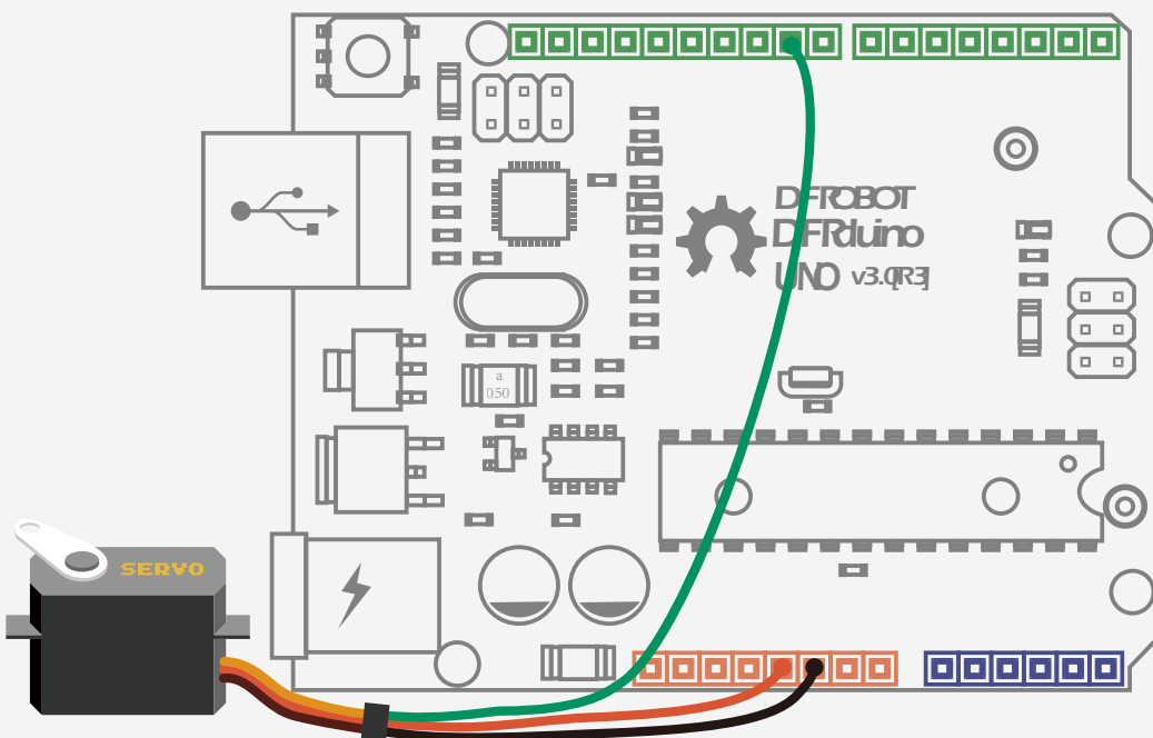
Circuit diagram of a servo connected to an Arduino
