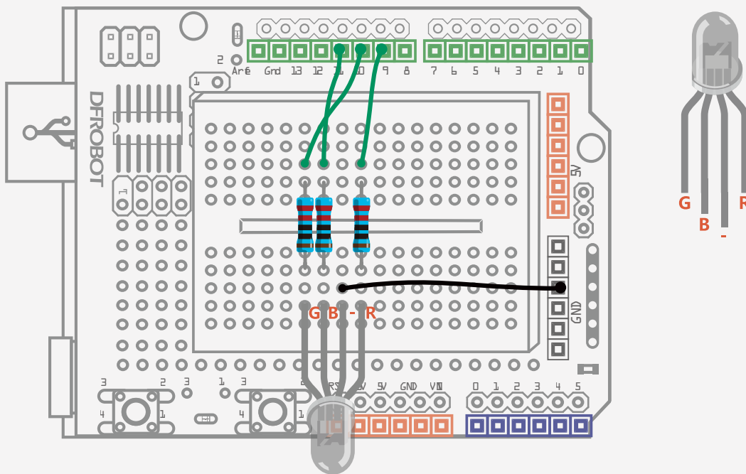
Fig. 5-1 Colourful RGB LED Diagram
