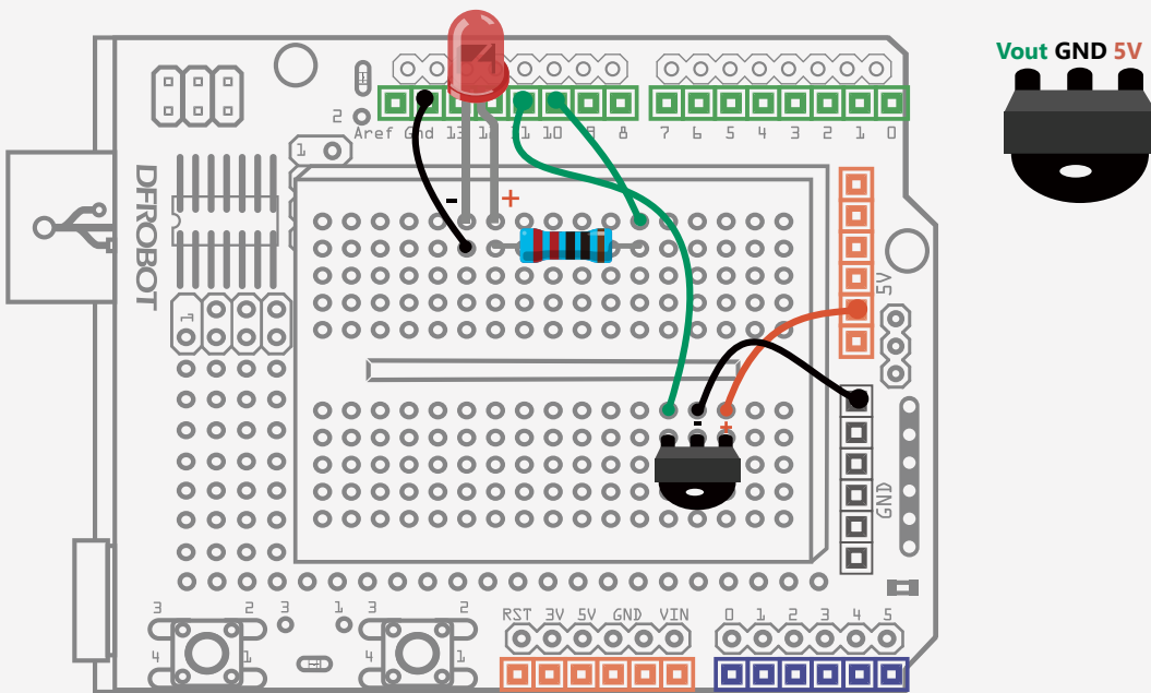
Fig. 14-2 IR Remote Controlled LED Circuit Diagram
