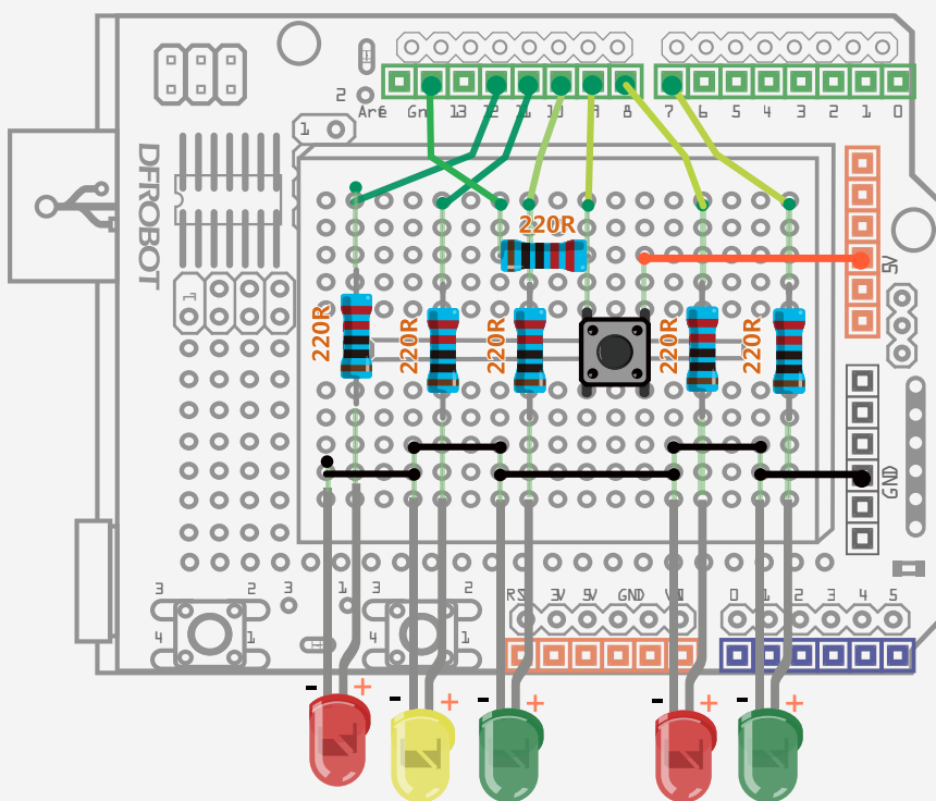
Fig 3-1 Wiring Diagram of LED Blinking
