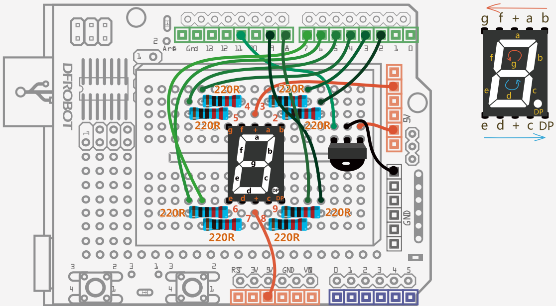
Fig. 15-3 IR Remote Controlled LED Module Diagram
