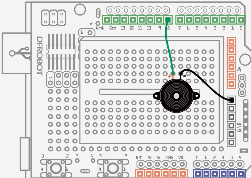
Fig. 6-1 Alarm Diagram
