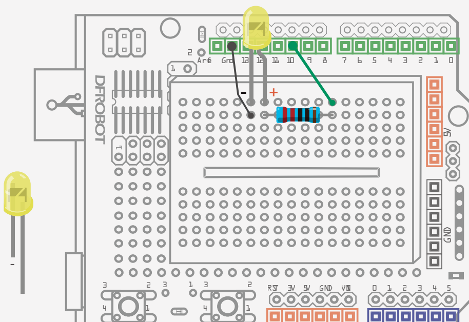
Fig 1-1 LED Flashing Circuit
