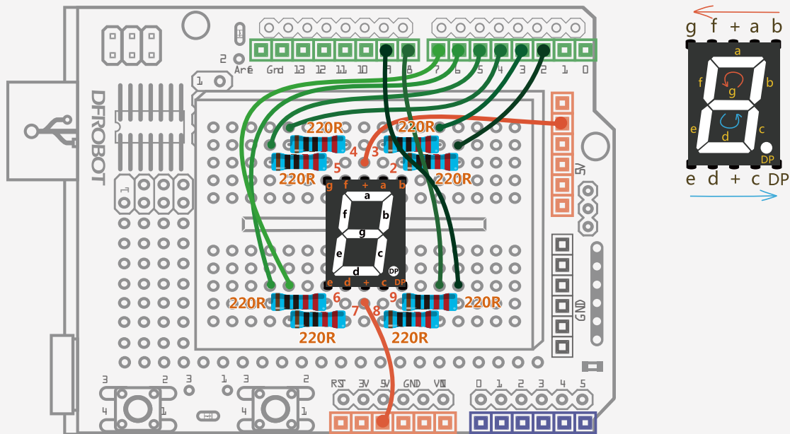
Fig. 15-1 LED Module Display Circuit Diagram
