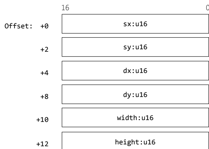
Copyarea Command Packet:
