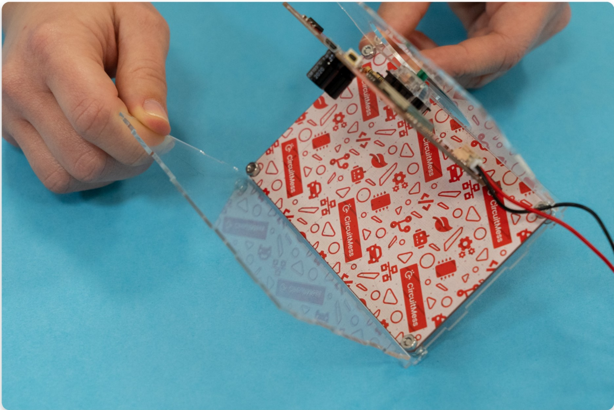
Connect the bottom casing layer
