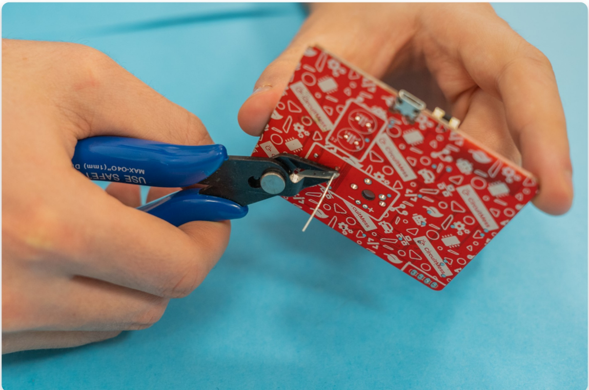
Cut the legs from the second resistor using your diagonal cutter pliers
