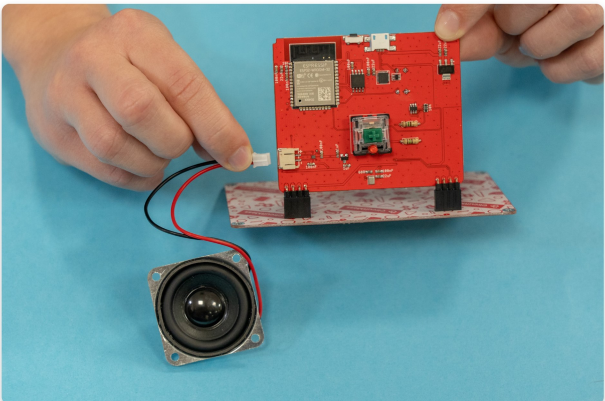
The correct way to connect the speaker
