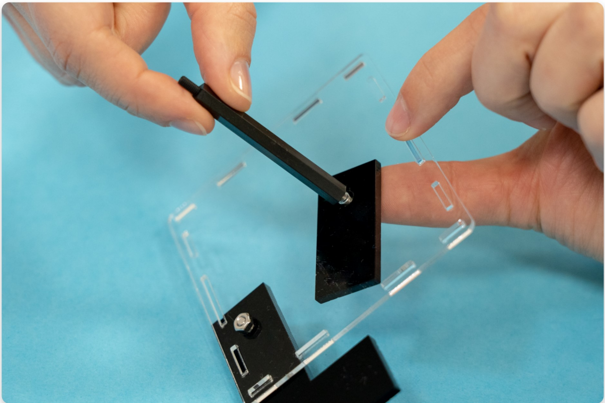
Fix the first long spacer
