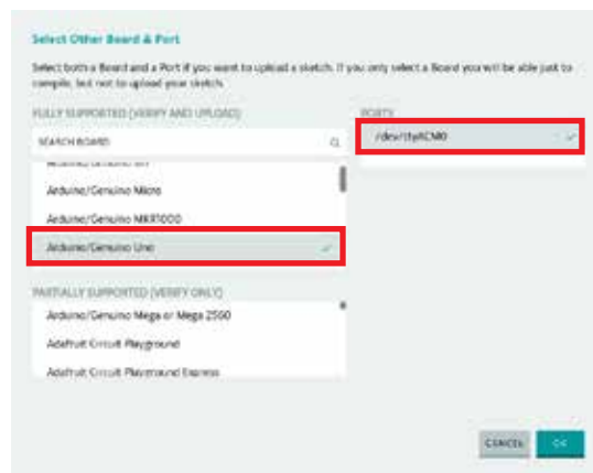
Selecting Board and Port on Chrome OS
