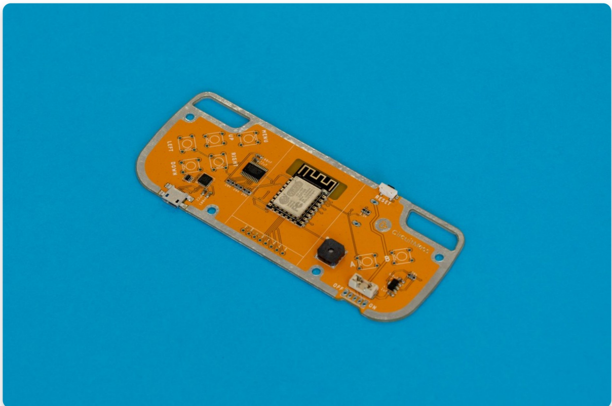
Front side of the main board
